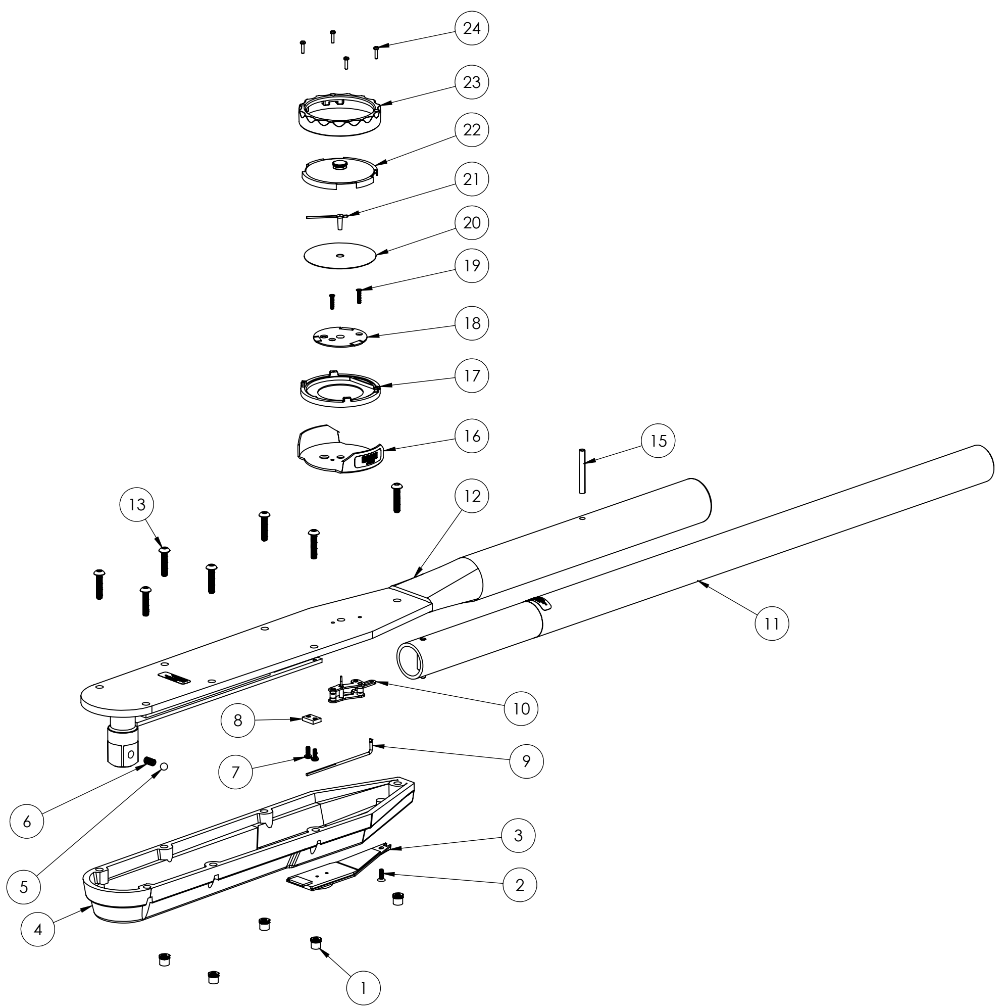
D4-600F 600 FT-LB MECHANICAL DIAL TORQUE WRENCH
