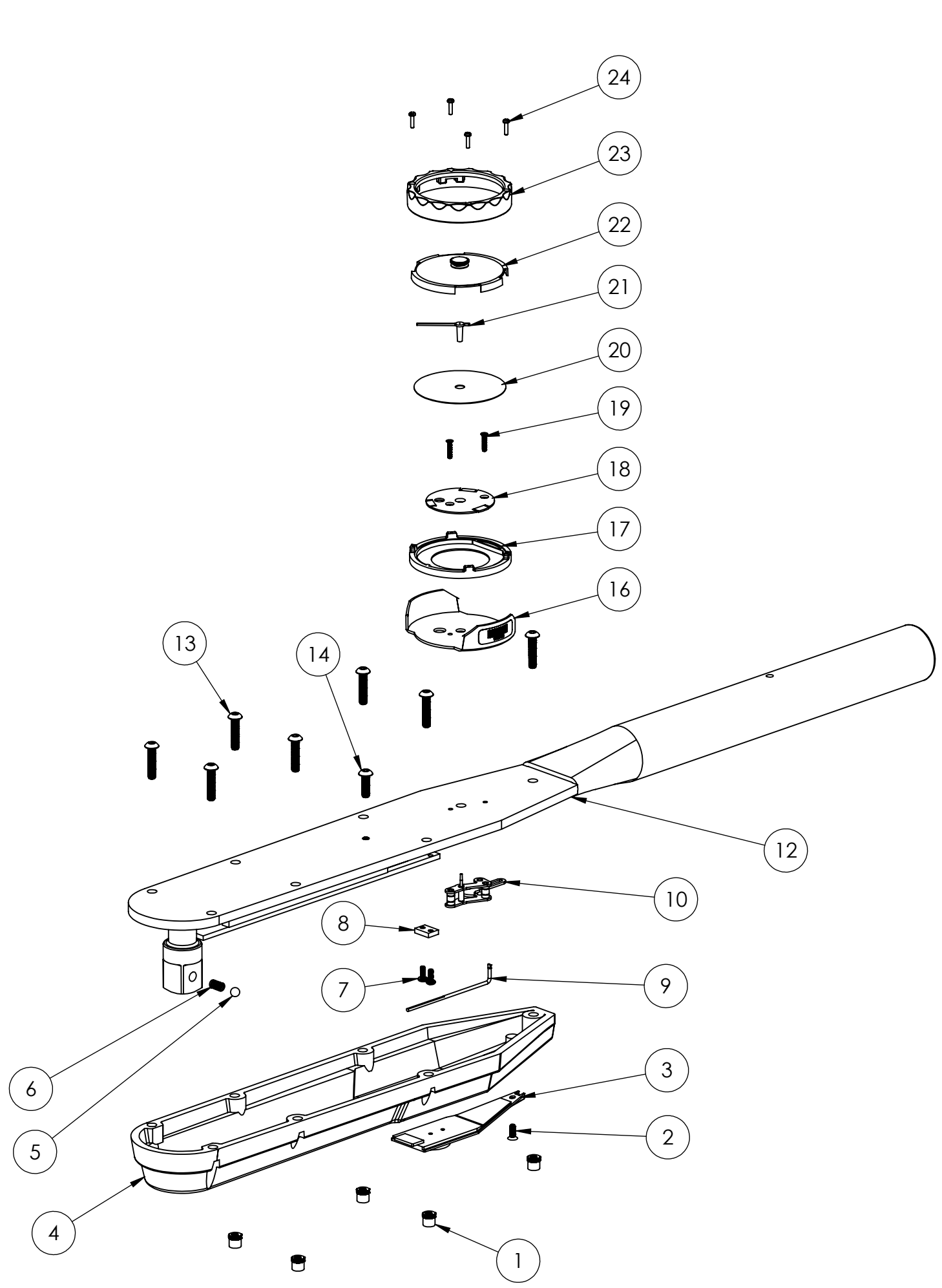
D4-350F 350 FT-LB MECHANICAL DIAL TORQUE WRENCH
