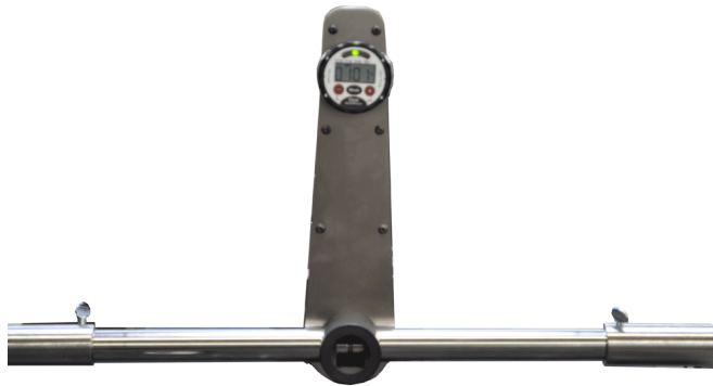
2000 ft.lb. Torque wrench shown with 5 Extensions (two man use)
